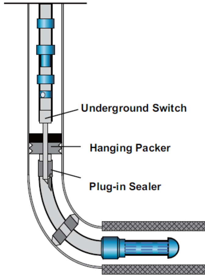
Steaming injection
